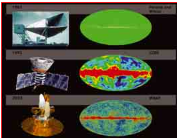
Cosmic background radiation, one of the greatest proofs of the Big Bang, was discovered in 1965 and has also been studied by the COBE (1992) and WMAP (2003) space satellites.
