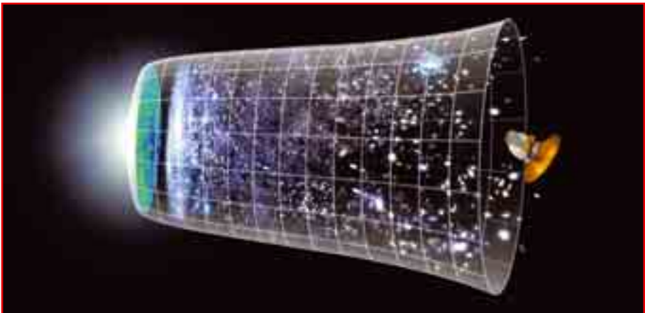
This image prepared from data from the WMAP satellite in 2006 represents the expansion of the universe from the first moment of the Big Bang to the present day.
